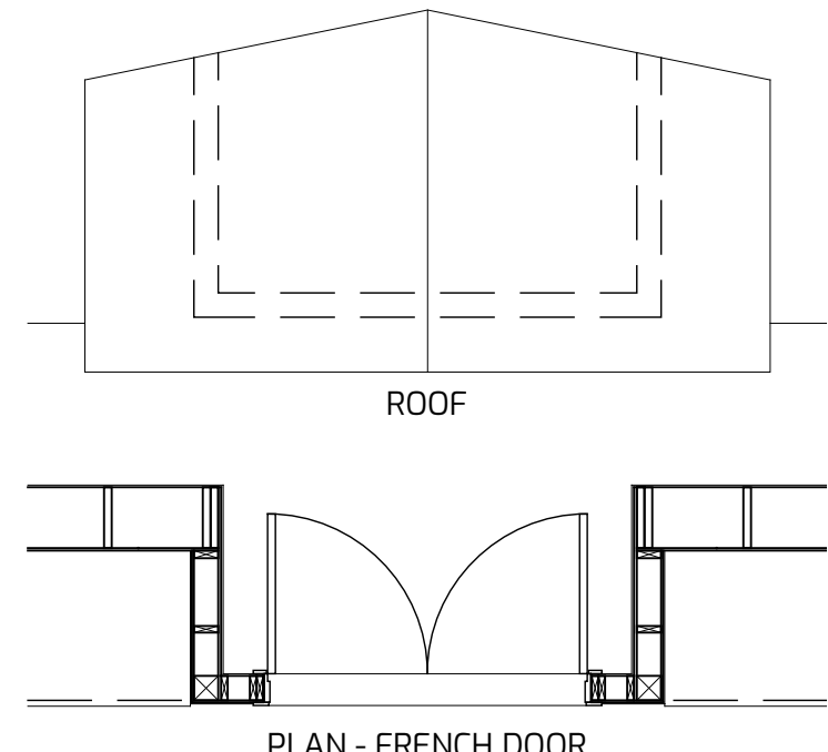
PLAN - FRENCH DOOR
