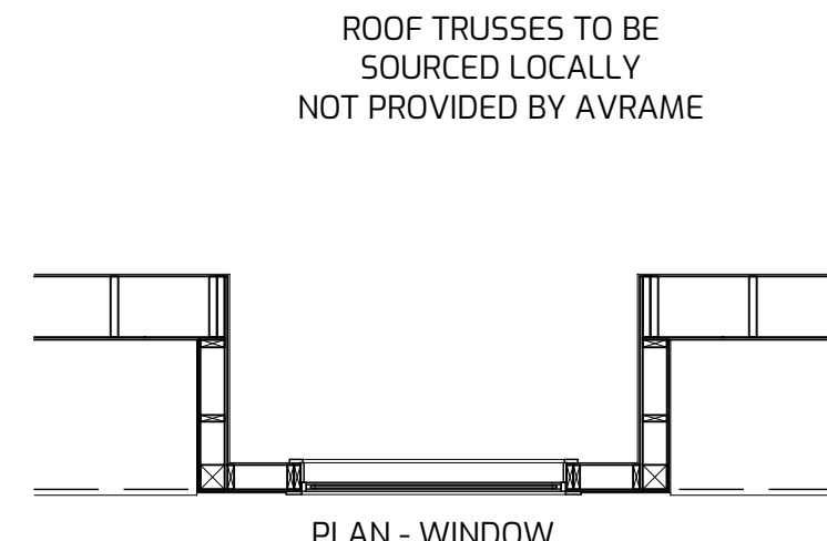
PLAN - WINDOW
