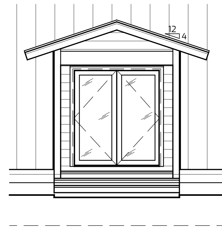
ELEVATION - FRENCH DOOR
