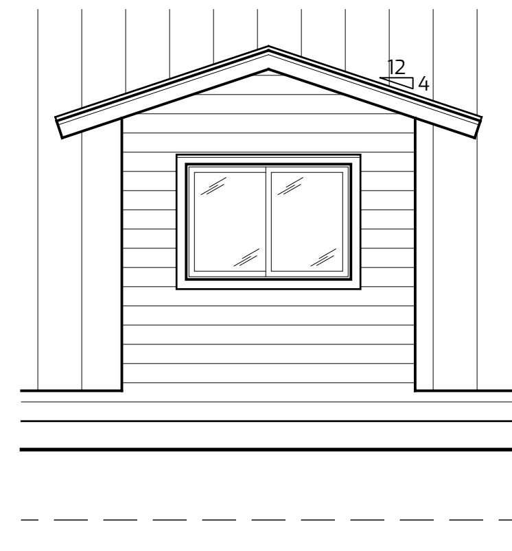
ELEVATION - WINDOW
