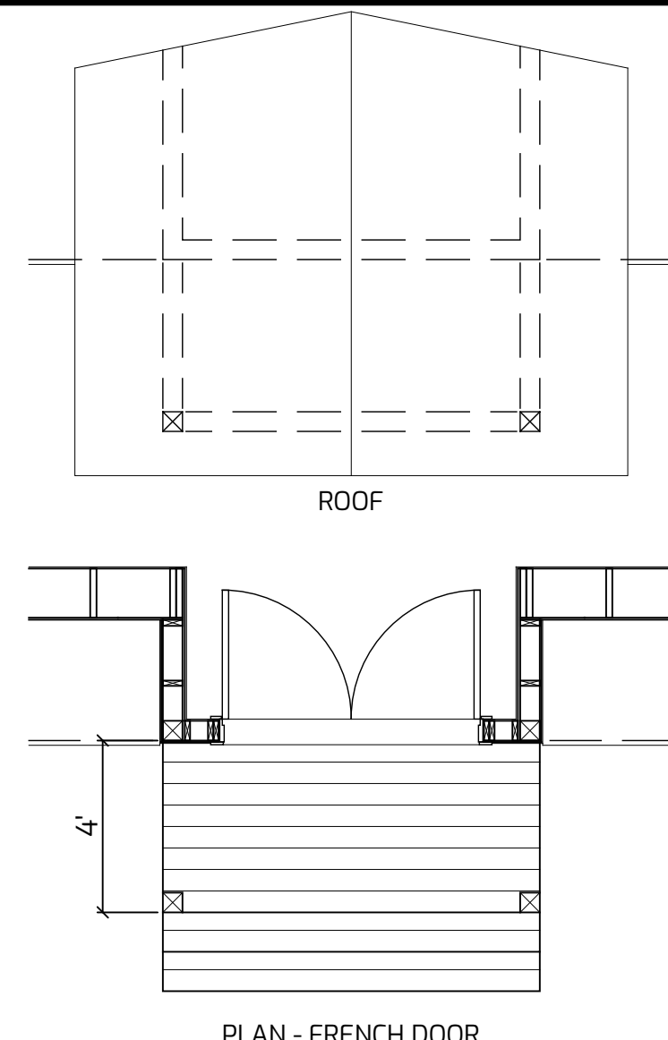
PLAN - FRENCH DOOR
