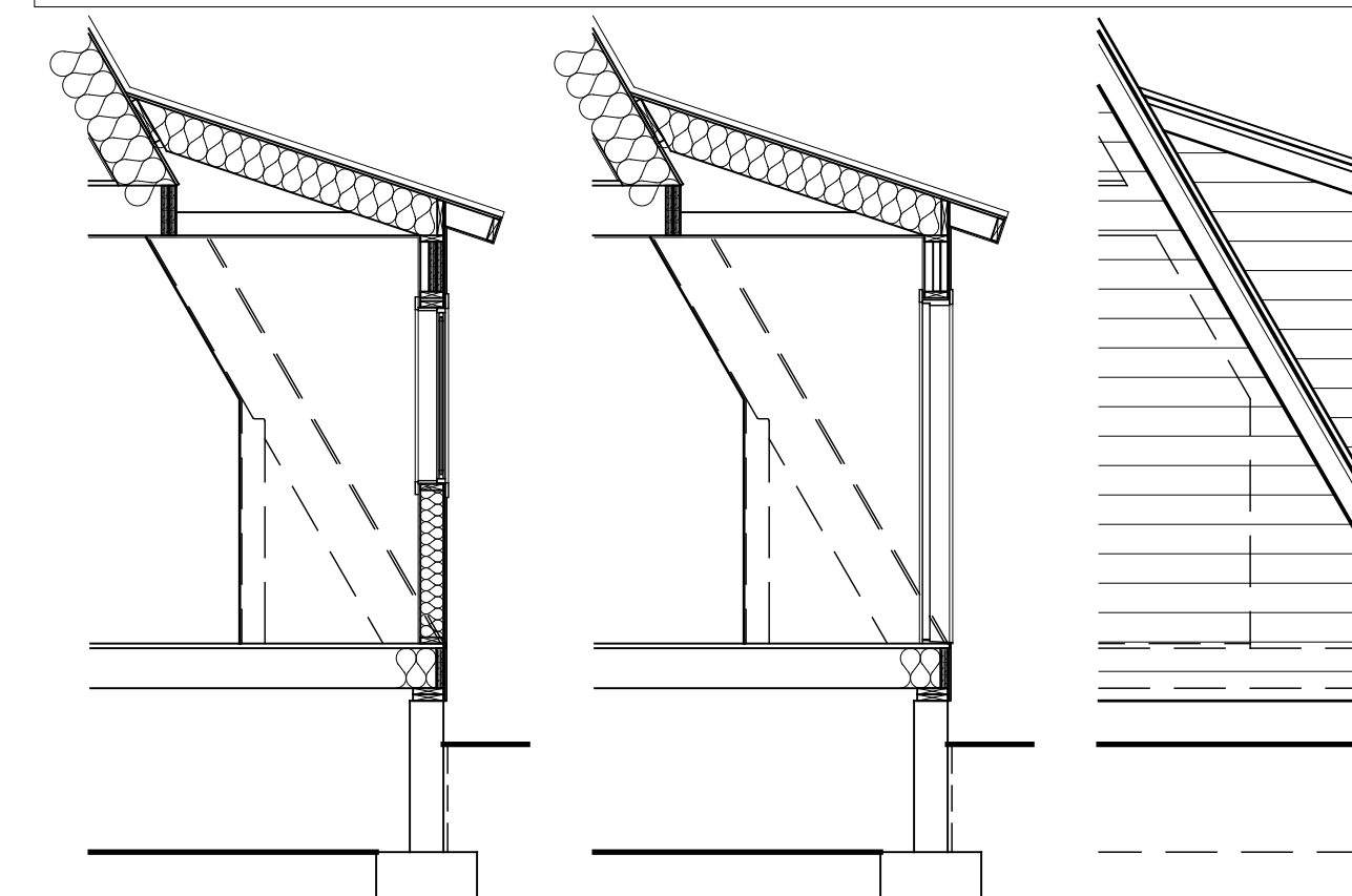
SECTION - WINDOW
