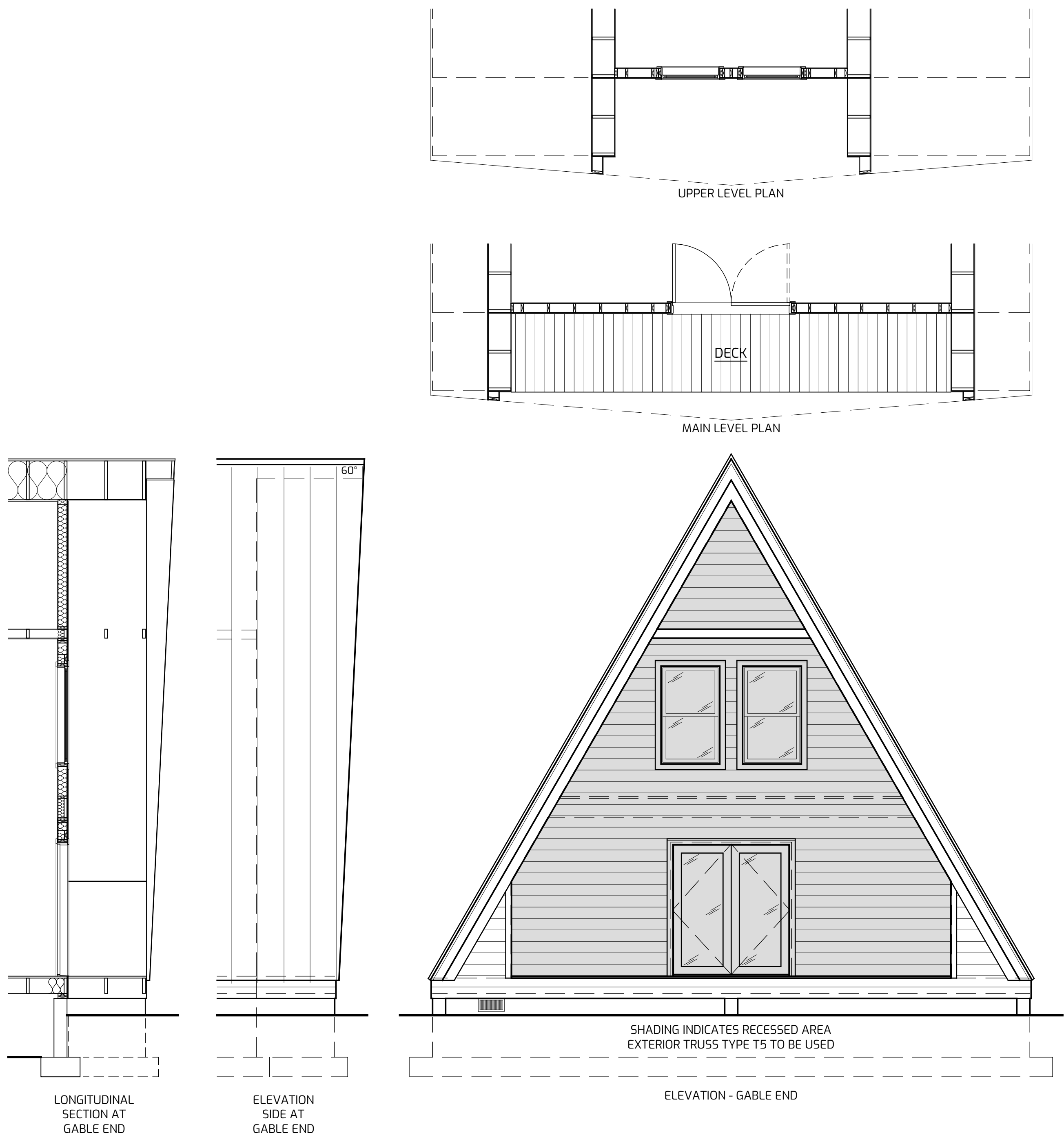
EXTENDED GABLE ROOF W/ MAIN LEVEL DECK
