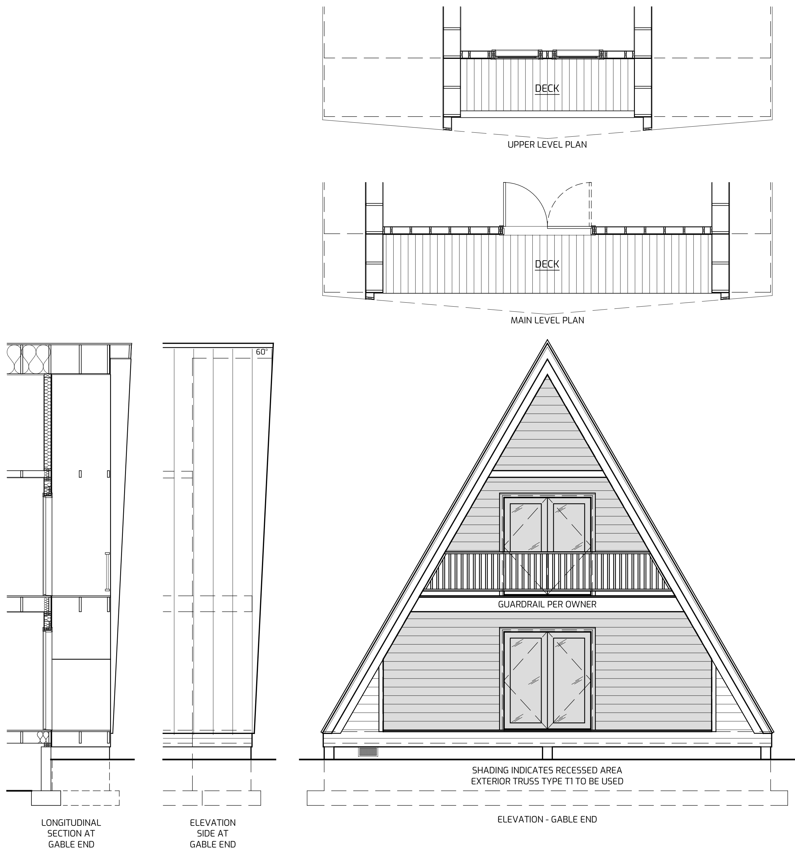
EXTENDED GABLE ROOF W/ MAIN & UPPER LEVEL DECKS
